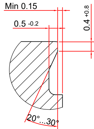
DETAIL B SCALE 8:1
