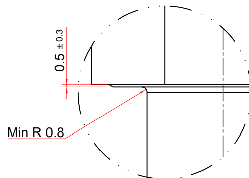
Detail B
